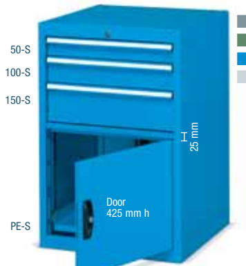
•ORD. NO. DRAWERS F DD 1175 51 04 3 Cabinet with 3 normal extension drawers 1 normal retractable shelf Dim. mm 564x726x850 h Central lock
