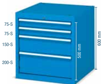
ORD. NO. DRAWERS F DD 1050 52 04 4 Cabinet with 4 normal extension drawers Dim. mm 564x726x600 h Central lock
