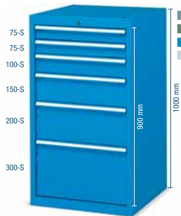
•ORD. NO. DRAWERS F DD 1090 52 04 6 Cabinet with 6 normal extension drawers Dimensions mm 564x726x1000 h Central lock
