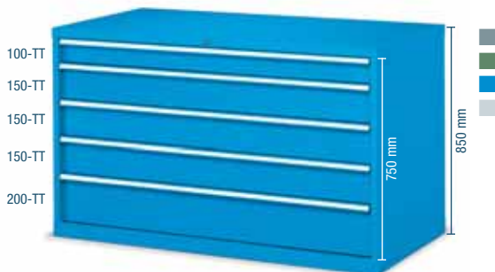
ORD. NO. DRAWERS F AG 7034 01 04 5 Cabinet with 5 full telescopic extension drawers Dimensions mm 1431x726x850 h Central lock
