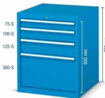
• ORD. NO. DRAWERS F DD 1060 54 04 4 Cabinet with 4 normal extension drawers Dim. mm 564x726x700 h Central lock
